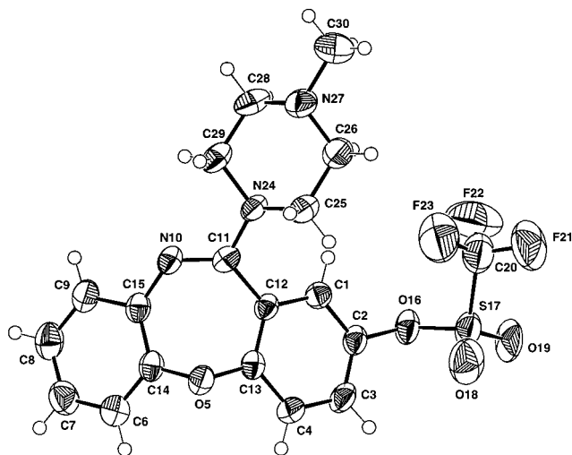
Figure 1. Molecular structure of compound 18a , showing 50% probability thermal ellipsoids for the non-H atoms and the atom-numbering scheme.
